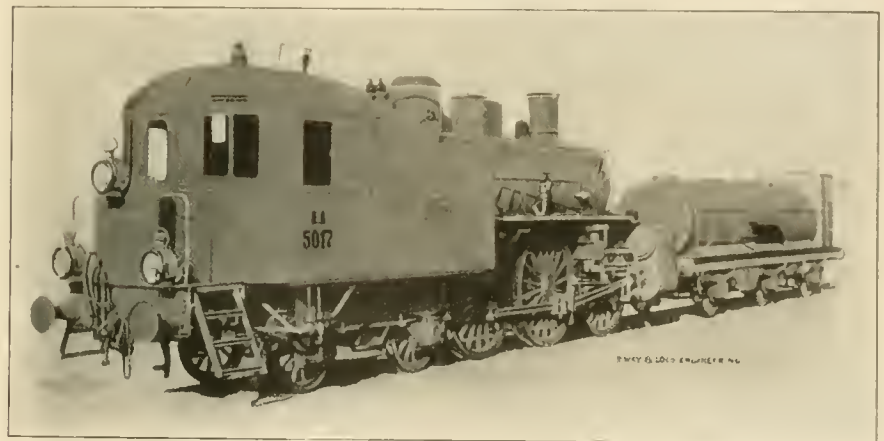
ENGINE RUNS CAB FIRST—ADRIATIC RAILWAY OF ITALY.
